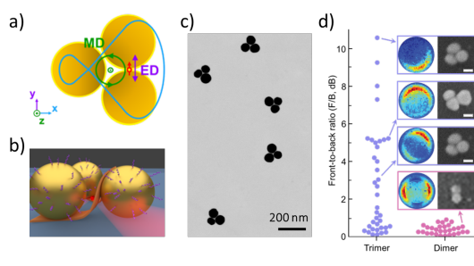
Figure 1. a) Configuration of the trimer nanoantenna driven by a single emitter (red arrow). The unidirectional radiation pattern (blue contour) stems from the balanced interference of the electric dipole (ED) and magnetic dipole (MD). b) A schematic showing how the curved origami template brings the single emitter to the dimer gap. c) An SEM image of the DNA origami-assisted trimer nanoantennas. d) Representative emission patterns and SEM images of trimer and dimer antennas. Distinct directionality (F/B ratio in dB) is found between trimers (purple dots) and dimers (pink dots).
